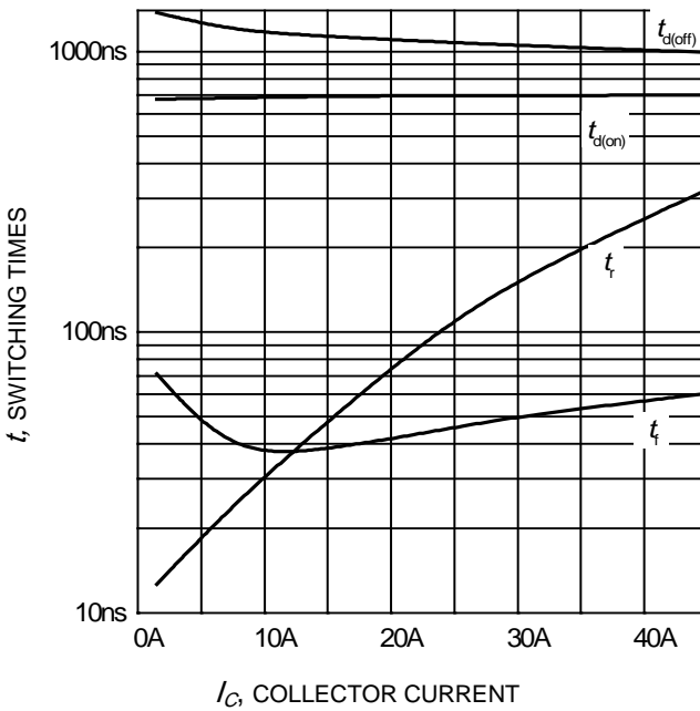
Figure 3. Typical switching times as a function of collector current (inductive load, T_{vj}=150^\circ\text{C} , V_{CE} = 300\text{V} Dynamic test circuit in Figure E)
