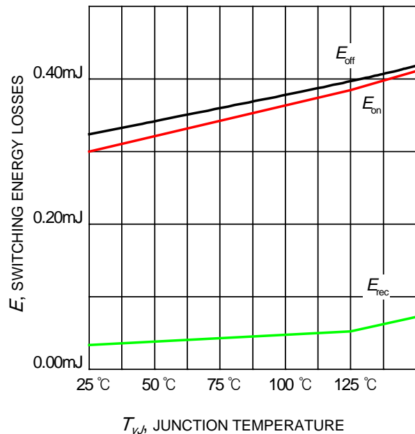
Figure 6. Typical switching energy losses as a function of junction temperature (inductive load, V_{CE} = 300\text{V} , I_C = 15\text{A} Dynamic test circuit in Figure A)
