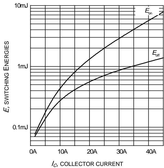
Figure 4. Typical switching energies as a function of collector current (inductive load, T_{vj} = 150^\circ\text{C} , V_{CE} = 300\text{V} Dynamic test circuit in Figure E)
