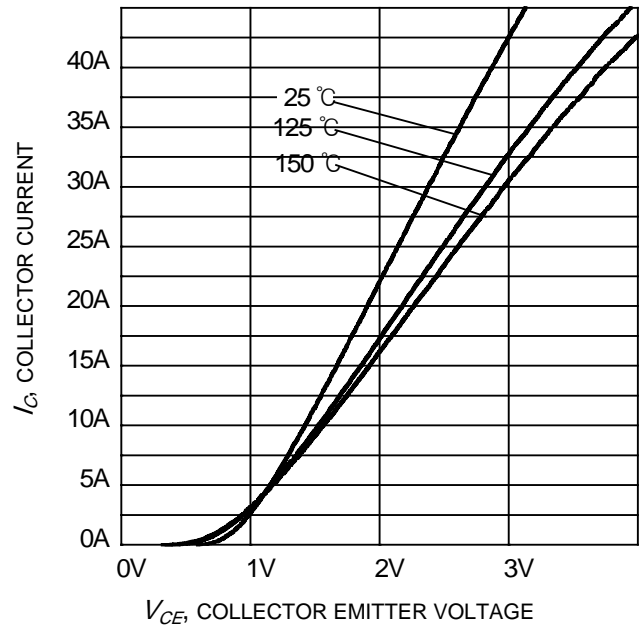
Figure 8. Typical IGBT output characteristic ( V_{DD} = 15V )
