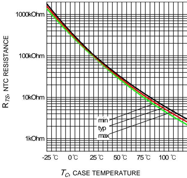
Figure 7. Typical NTC characteristic as a function of NTC temperature
