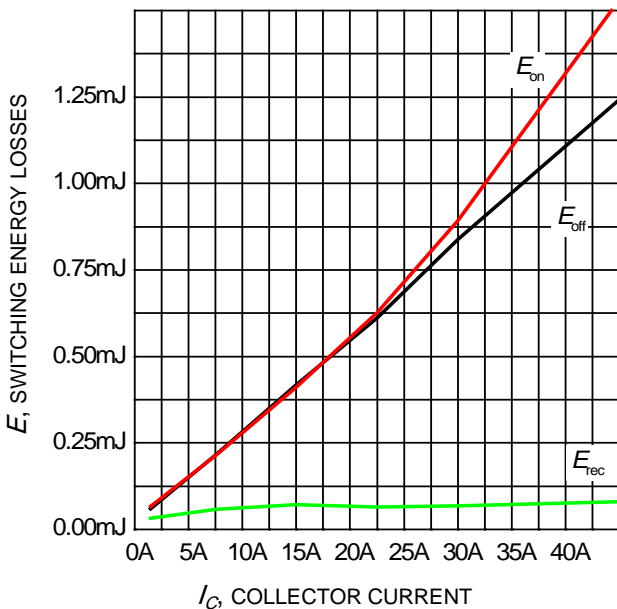
Figure 5. Typical switching energy losses as a function of collector current (inductive load, T_{vj} = 150^\circ\text{C} , V_{CE} = 300\text{V} Dynamic test circuit in Figure A)
